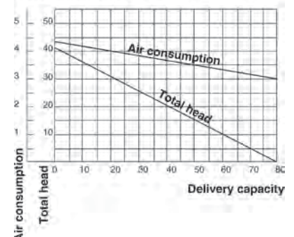
Performance curve YP-35
